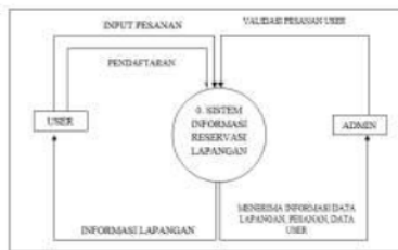
Picture 3.2 DFD Level 0
